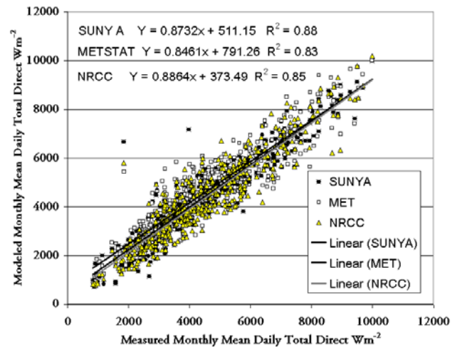
Fig. 3. Modeled versus measured DNI monthly mean daily totals, regression fit, and correlation coefficients by model
