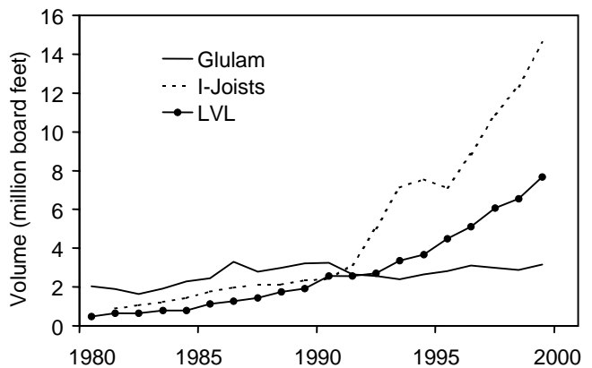
Figure 9—Production of glulam, I-joists, and laminated veneer, 1965–1999.
