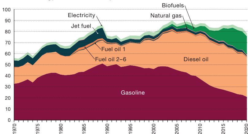
Final energy use in the transport sector, domestic, 1970–2020, TWh
