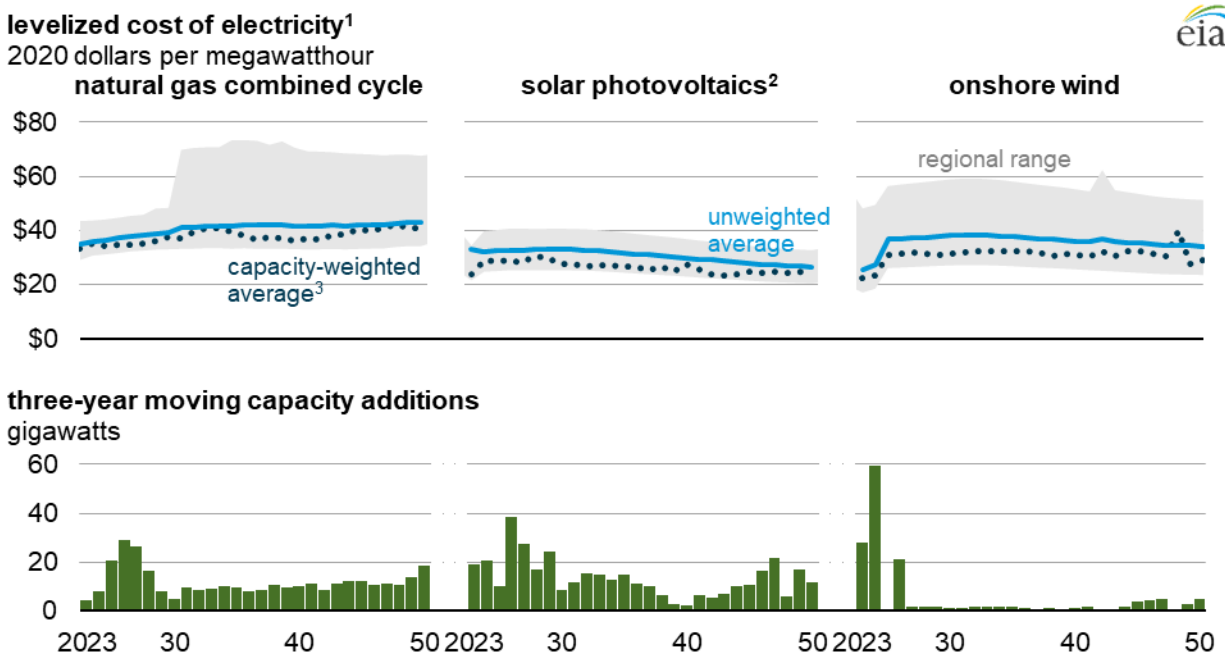
Figure 3. Capacity-weighted and unweighted levelized cost of electricity (LCOE) projections and three-year moving capacity additions for selected generating technologies, 2023–50
