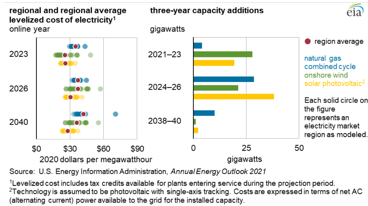
Figure 1. Levelized cost of electricity (with applicable tax subsidies) by region and total incremental capacity additions for selected generating technologies entering into service in 2023, 2026, and 2040
