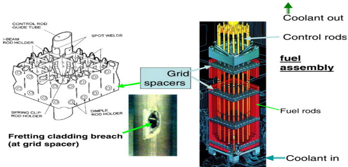
Figure Grid-to-Rod failure
