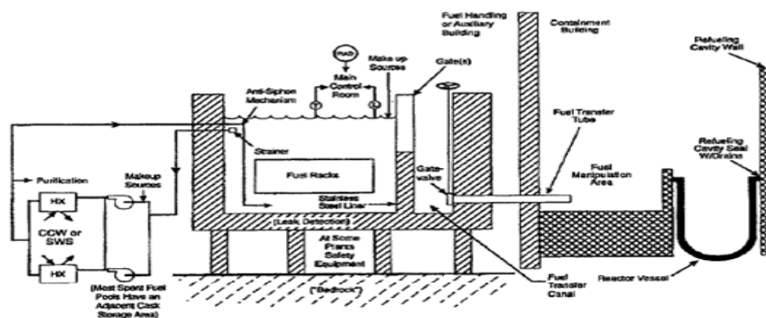
Figure 6. Layout for spent fuel pool and transfer system for pressurized water reactors
