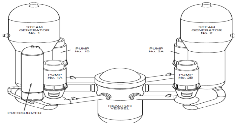
Figure 2 the SONGS Reactor Design
