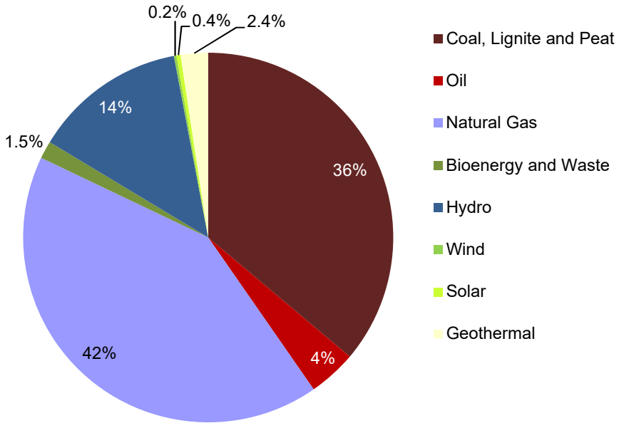
FIGURE 58. ELECTRICITY PRODUCTION BY ENERGY SOURCE IN THE SOUTH-EASTERN ASIA REGION IN 2016
