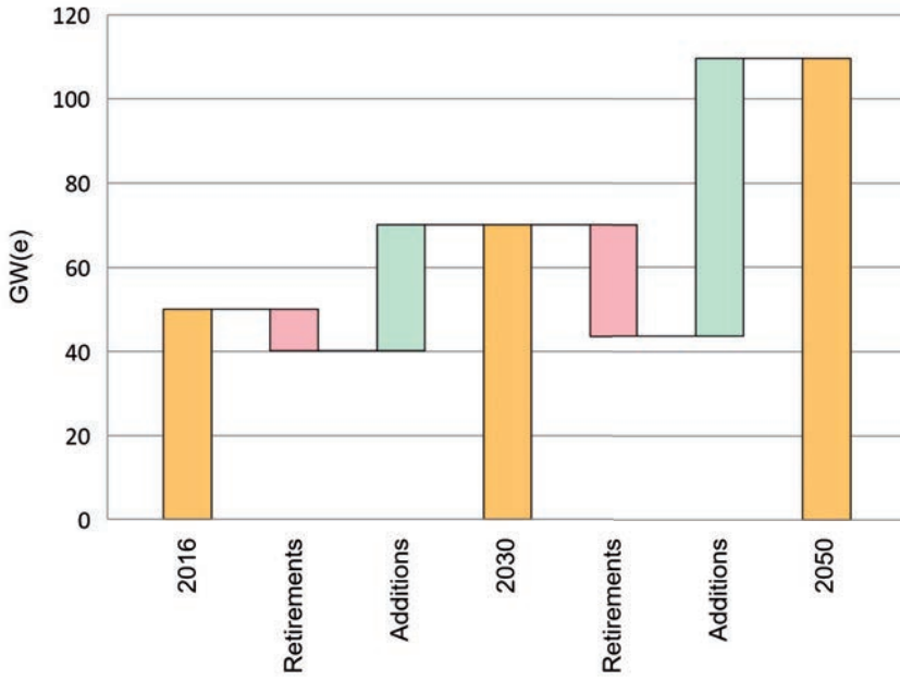
FIGURE 31. NUCLEAR CAPACITY IN THE EASTERN EUROPE REGION: ACTUAL, RETIREMENTS AND ADDITIONS
