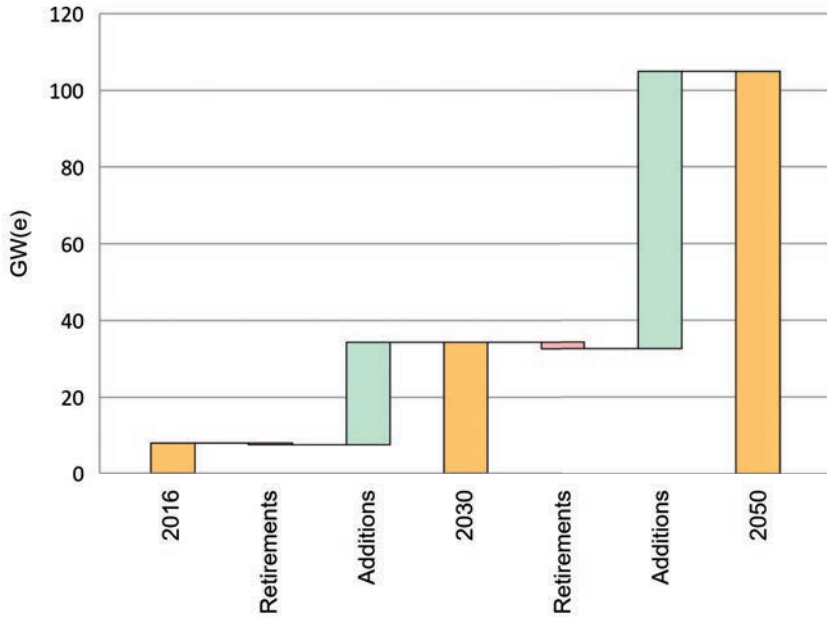
FIGURE 49. NUCLEAR CAPACITY IN THE SOUTHERN ASIA REGION: ACTUAL, RETIREMENTS AND ADDITIONS
