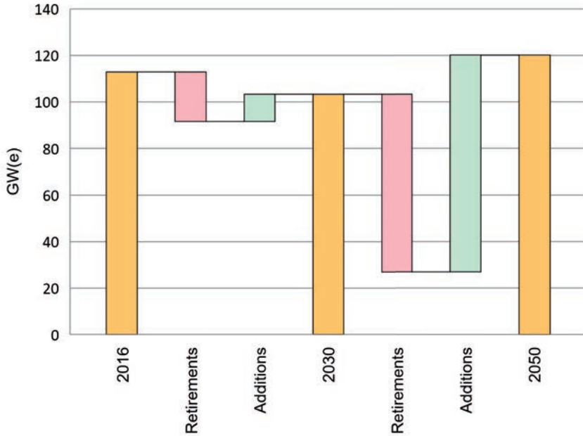
FIGURE 25. NUCLEAR CAPACITY IN THE COMBINED REGIONS OF NORTHERN, WESTERN AND SOUTHERN EUROPE: ACTUAL, RETIREMENTS AND ADDITIONS
