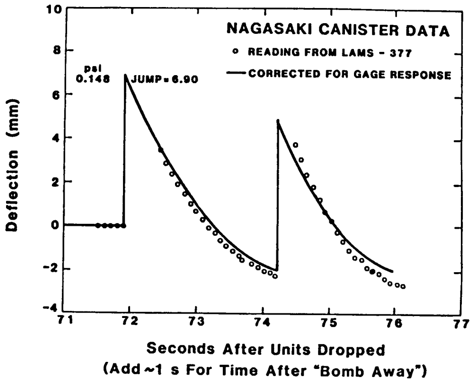
Fig. 2. Nagasaki canister pressure data.
