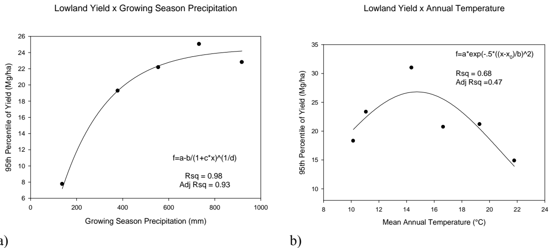
a) b) Fig. 19. Regressions through the 95 th percentile of lowland ecotype yield, as a function of (a) growing season precipitation and (b) annual temperature intervals as described in the text. In the legend of panel (b), a represents r and b represents s as defined in Eq. 2. The form of the equation and R^2 values are shown on the plots.
