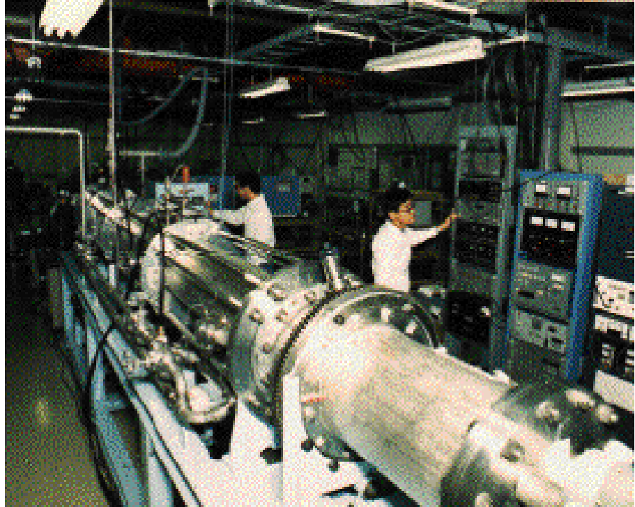
Figure 3-15. Highpower 16 \mu m Laser System for RIMLIS
