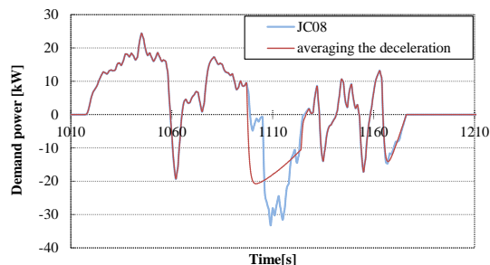
Figure 11: The comparison of the demand brake power
