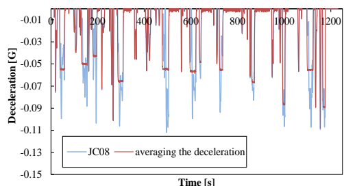
Figure 8: Deceleration
