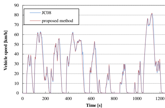
Figure 14: Vehicle speed
