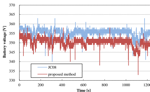
Figure 17: Battery voltage
