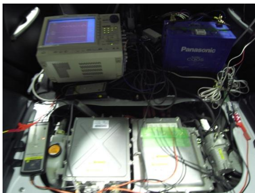
Figure 13: Battery of “i-MiEV”
