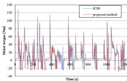
Figure 16: Motor torque
