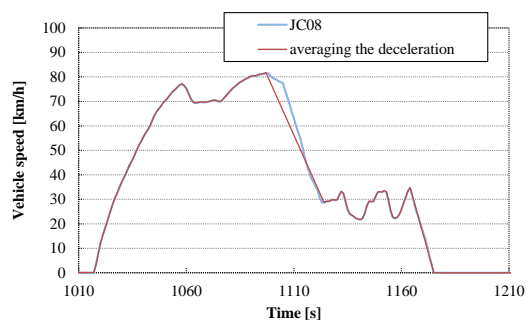
Figure 9: The comparison of the vehicle speed
