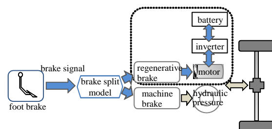
Figure 1: Brake system
