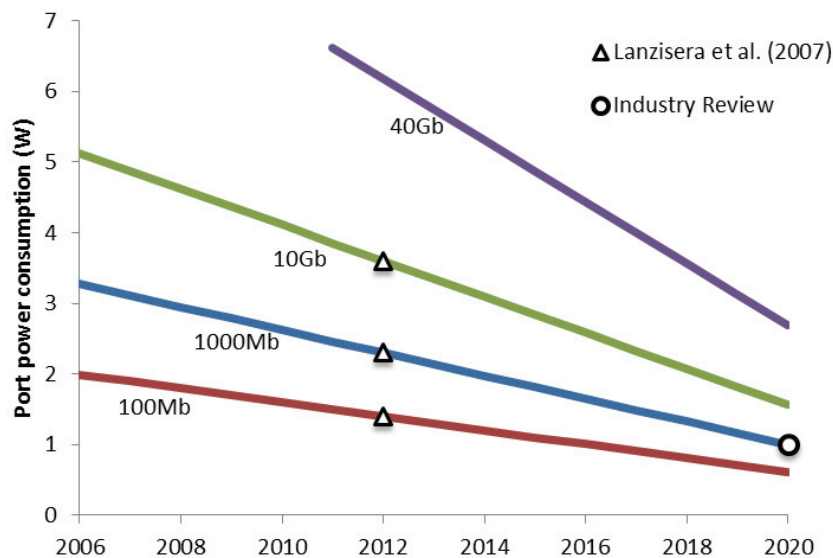
Figure 18. Assumed Network Power for Four Port Speeds
