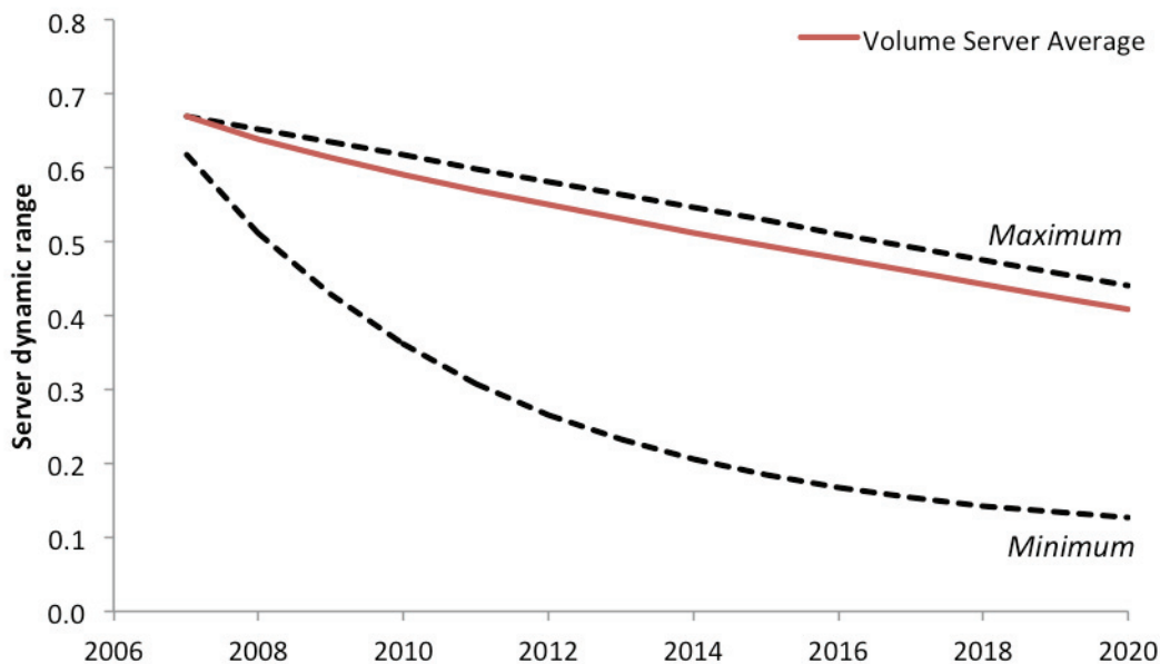
Figure 8. Assumed Dynamic Range of Volume Servers
