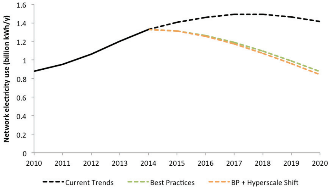
Figure 33. Network Electricity Use for Current Trends and Best Practices Scenarios. Improved Operation, Hyperscale Shift, and IO+HS scenarios are identical to Current Trends. BP+HS network electricity is slightly lower than BP alone due to the higher prevalence of network ports in hyperscale data centers where the 25% wattage reduction is assumed to occur.
