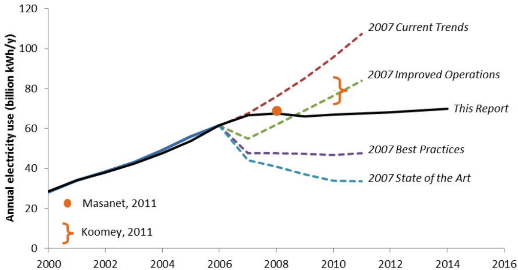
Figure 23. Historical Data Center Total Electricity Use
