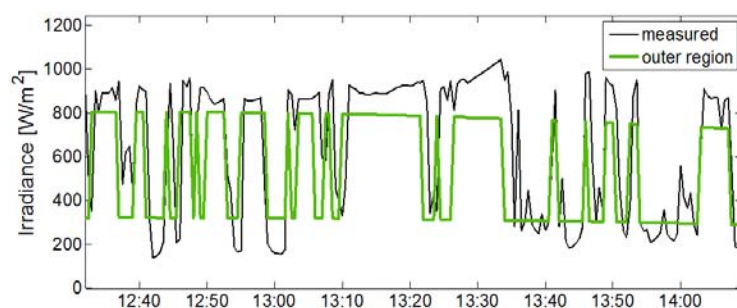
Figure 3b: 30 second GHI ramp forecast from the Total Sky Imager (green) against measurements by a 1 sec GHI station at the UC San Diego campus (black). Timing of cloudy-clear and clear-cloudy ramps on this day with cumulus clouds are accurately predicted with the sky imager.
