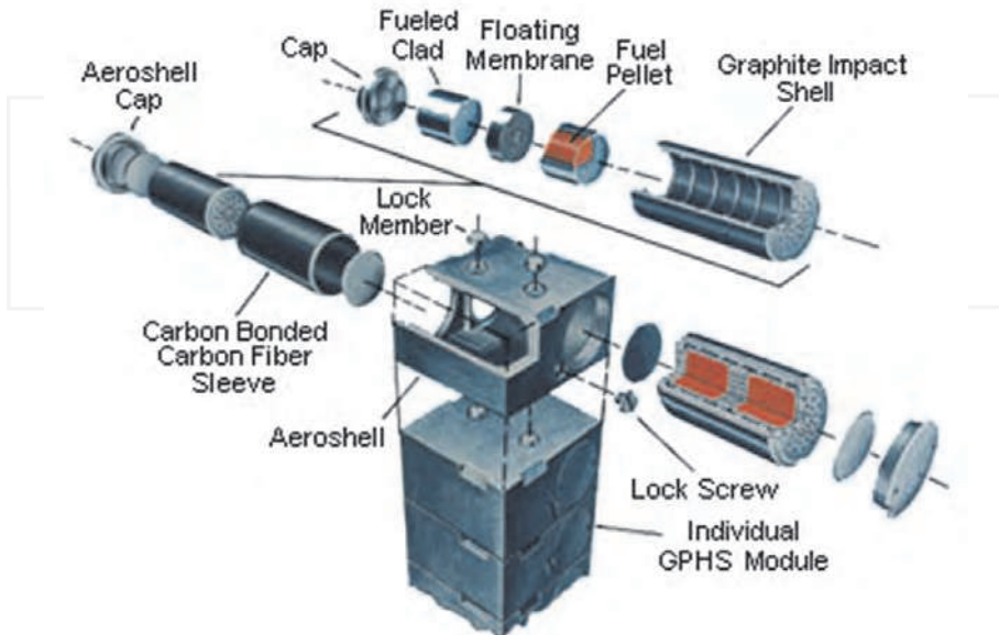
Fig. 3. GPHS module assembly.
