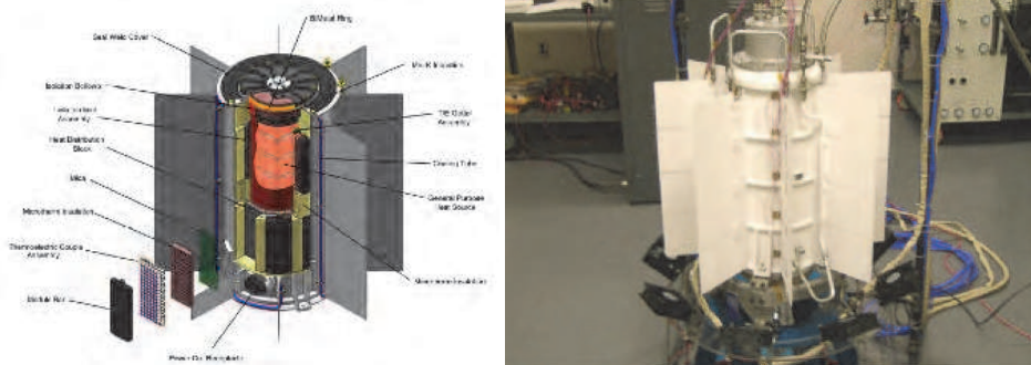
Fig. 27. Multi-Mission RTG (MMRTG). Cutaway schematic of power unit on left. MMRTG Qualification Unit undergoing tests on right.
