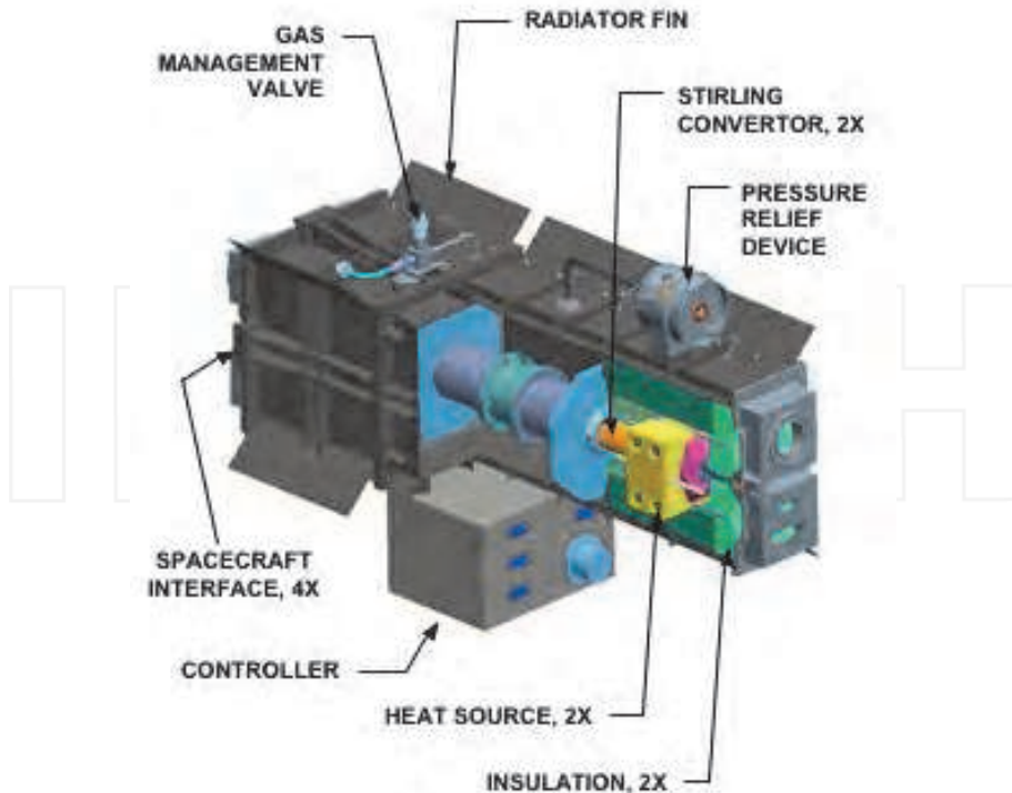
Fig. 30. Advanced Stirling Radioisotope Generator (ASRG).
