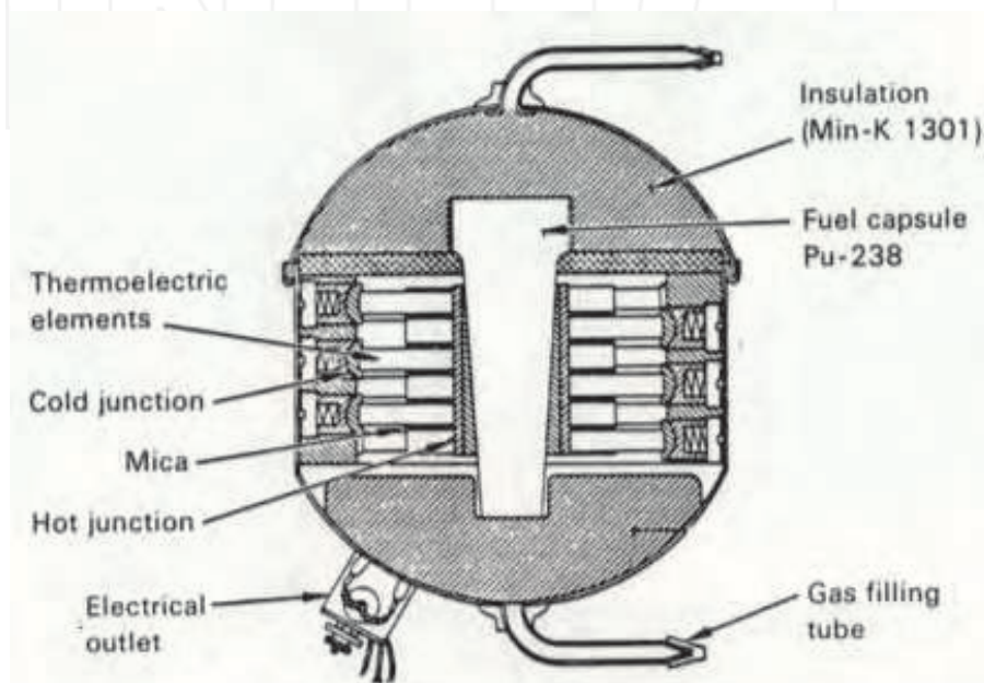
Fig. 6. SNAP-3B Schematic.
