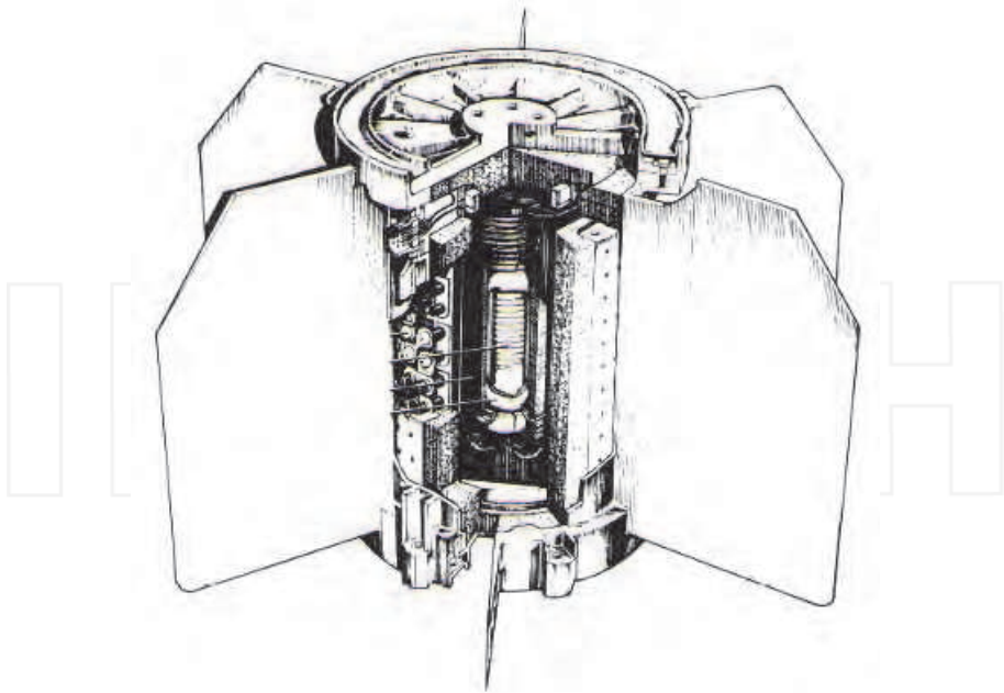
Fig. 11. Pioneer SNAP-19.
