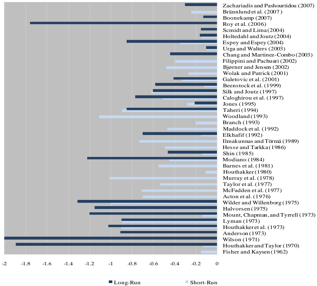
Figure 42. Comparison of Estimates of Price and Income Elasticity of Demand for Electricity Short- and Long-Run (a) Price (b) Income Elasticity Estimates
