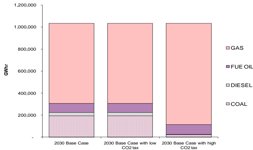
Figure 28. Sensitivity Analysis: CO 2 Tax. Composition Generation Mix (only fossil fuels)
