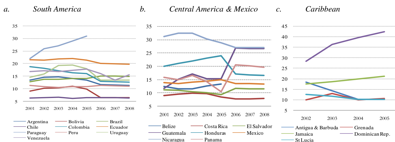
Figure 35. Total Distributional Electricity Losses in the LAC, %
