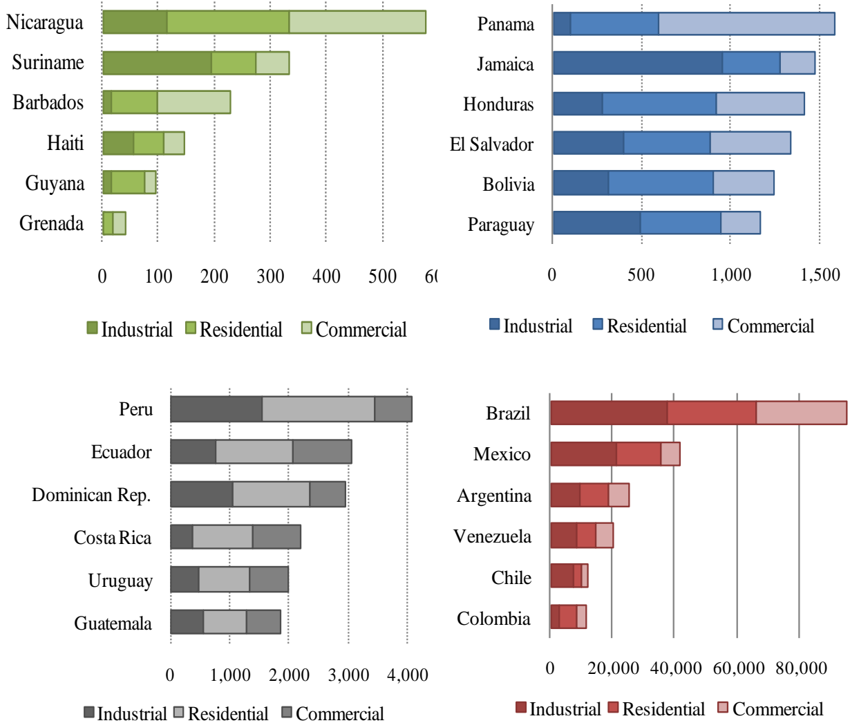
Figure 39. Extrapolating Argentina’s Efficiency Level: Annual Savings (GWh)
