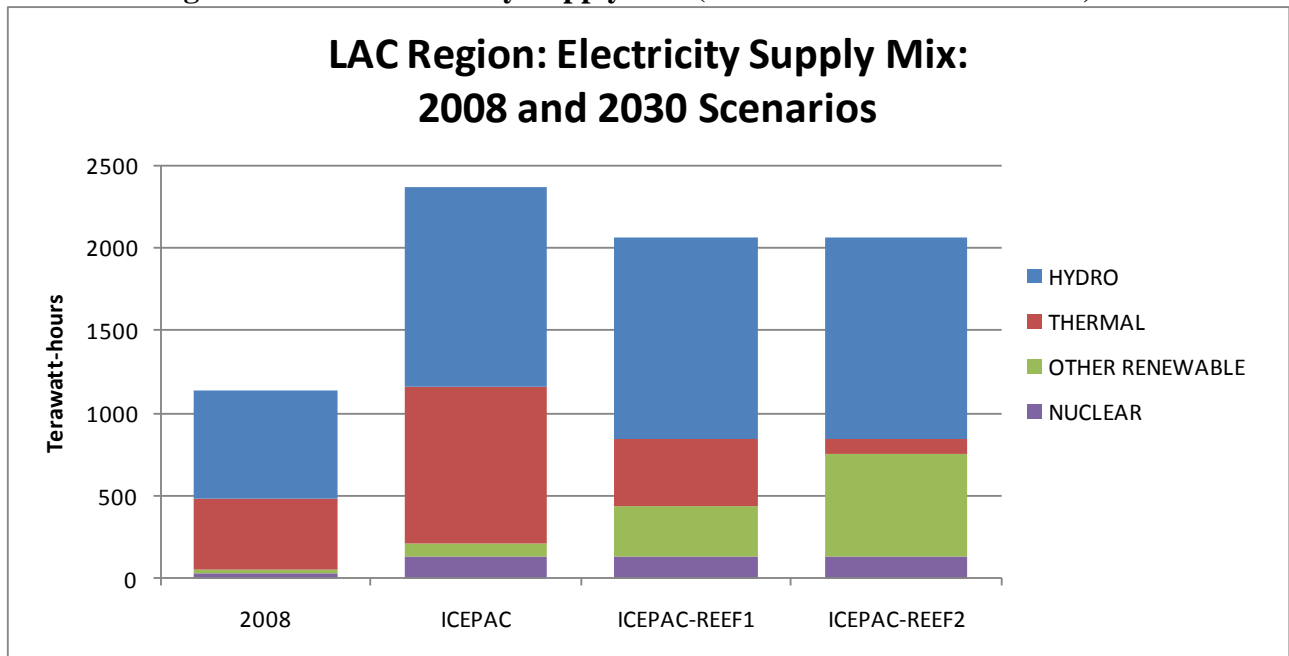
Figure 41. LAC Electricity Supply Mix (Various ICEPAC Scenarios)
