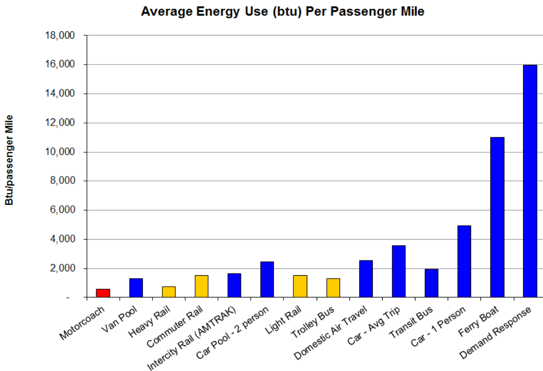
Figure 1.2 Energy Use (btu) per Passenger-Mile, by Mode
