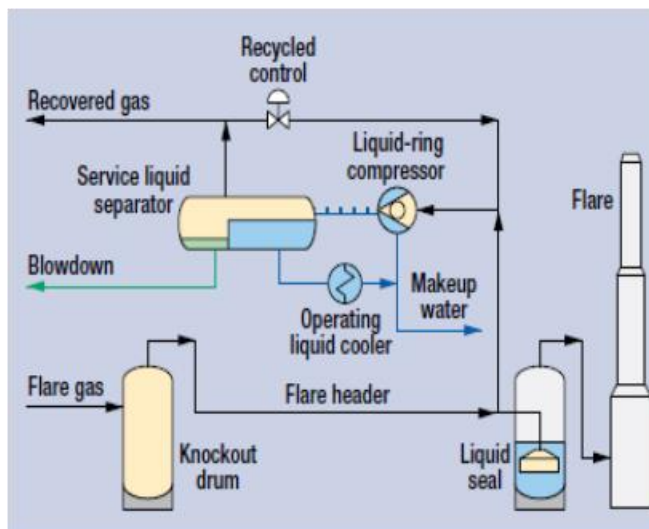
Figure 5 A view of a flare gas recovery system [48]
