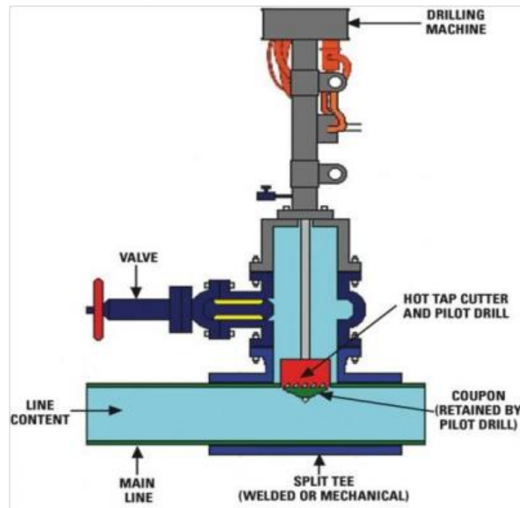
Figure 6. Hot tapping [16]
