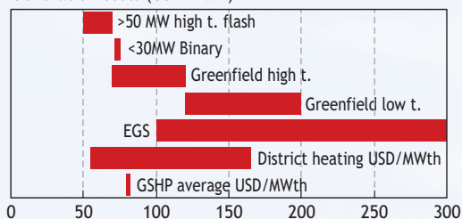
Figure 2. Generation costs
