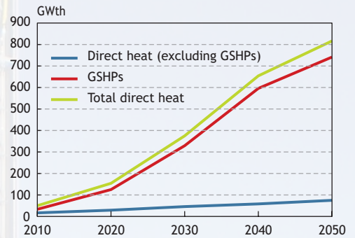
Figure 4. Geothermal direct use and GSHP capacity growth scenarios
