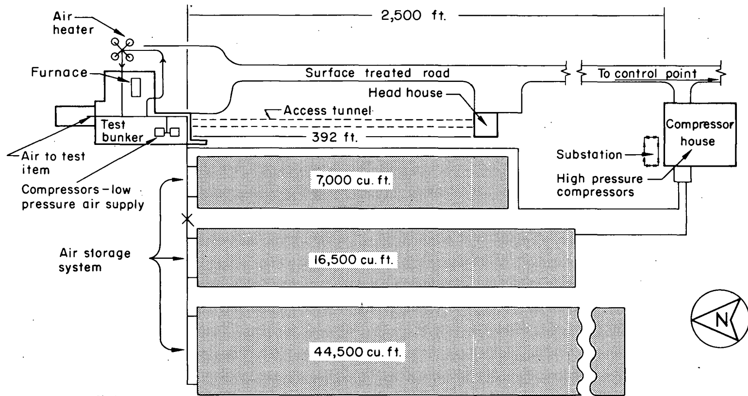
Fig. 2. Test area arrangement.
