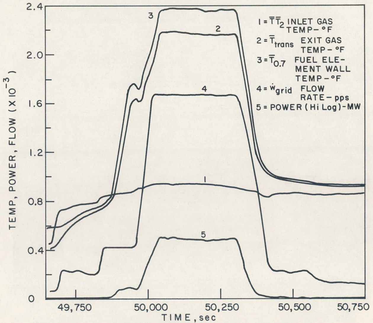
Fig. 6. Uncorrected major parameters during run 89.
