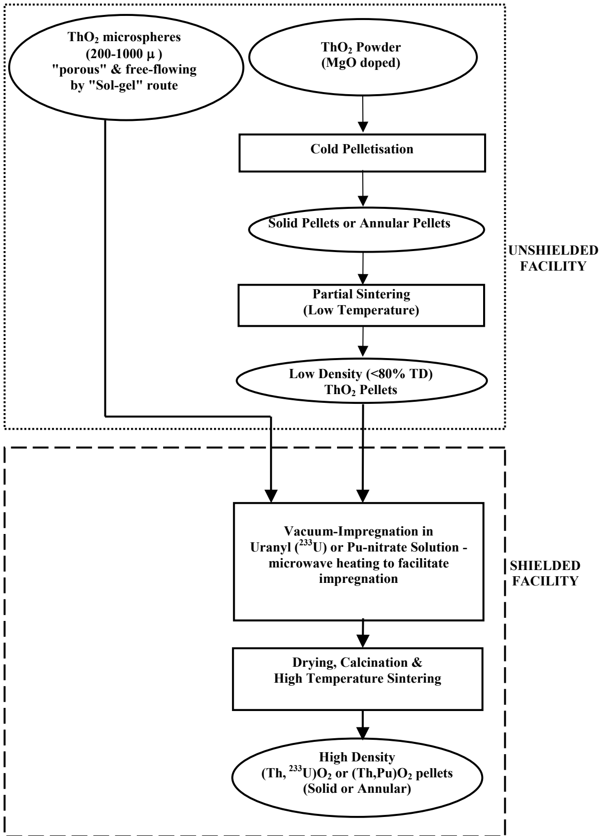
Fig. 19. Process flowsheet based on "Impregnation Technique" for manufacturing high density (Th, {}^{233}U)O_2 and (Th,Pu)O_2 fuel pellets.
