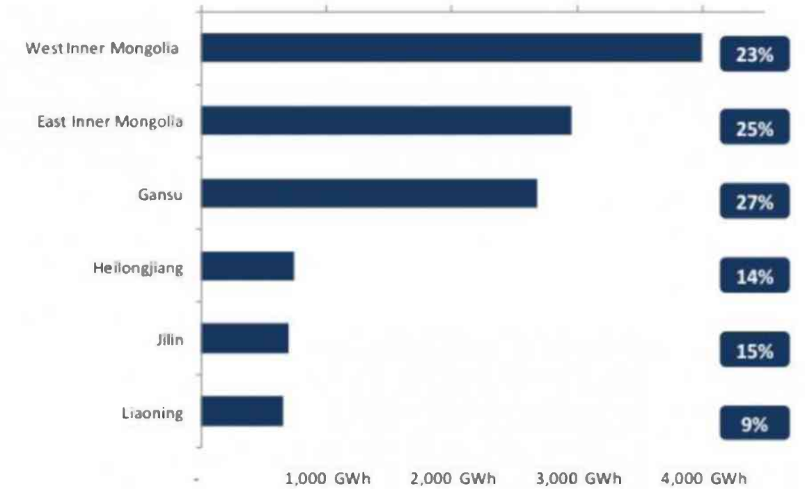
Figure 22: Curtailed wind generation and curtailed percent by province, 2011. Source: China State Electricity Regulatory Commission
