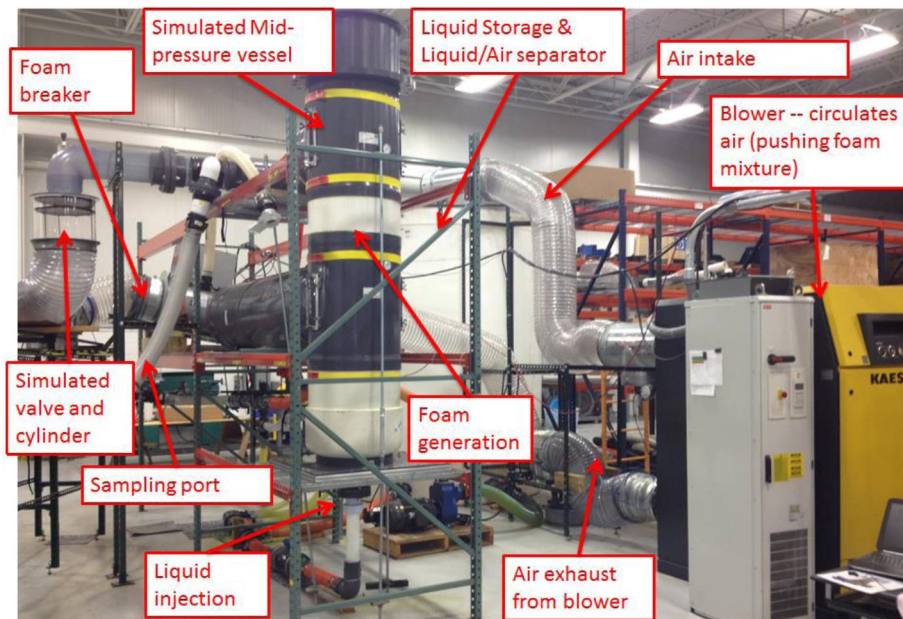
Figure 12: Foam generation and transport test stand, which mimics the mid-pressure vessel in our 1.5 MW ICAES system
