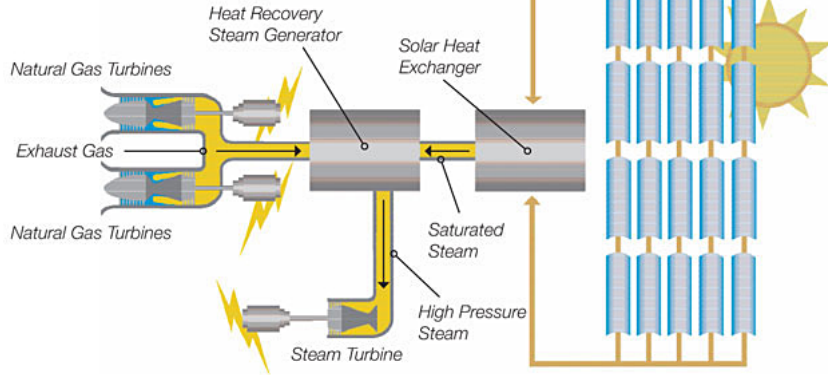
Figure 10. Rendering of a solar/fossil hybrid facility
