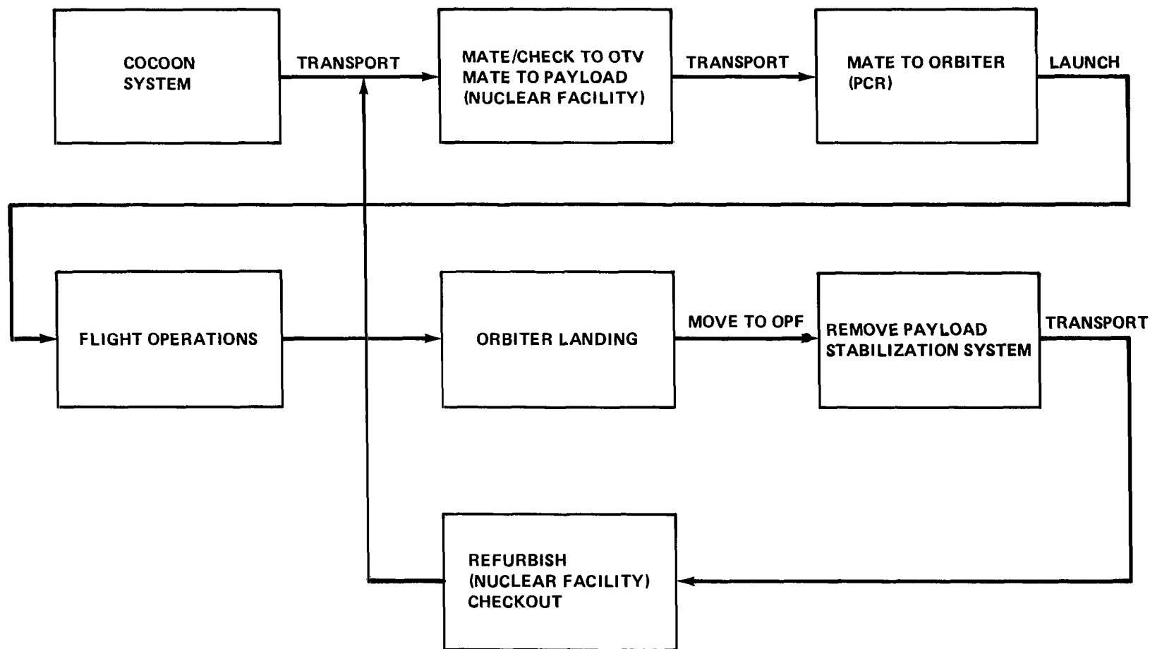
Figure 30. Cocoon flow.
