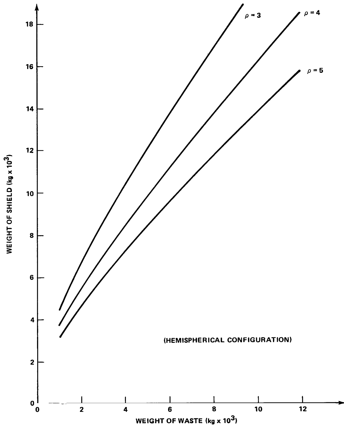
Figure 20. Shield weight as a function of waste density.
