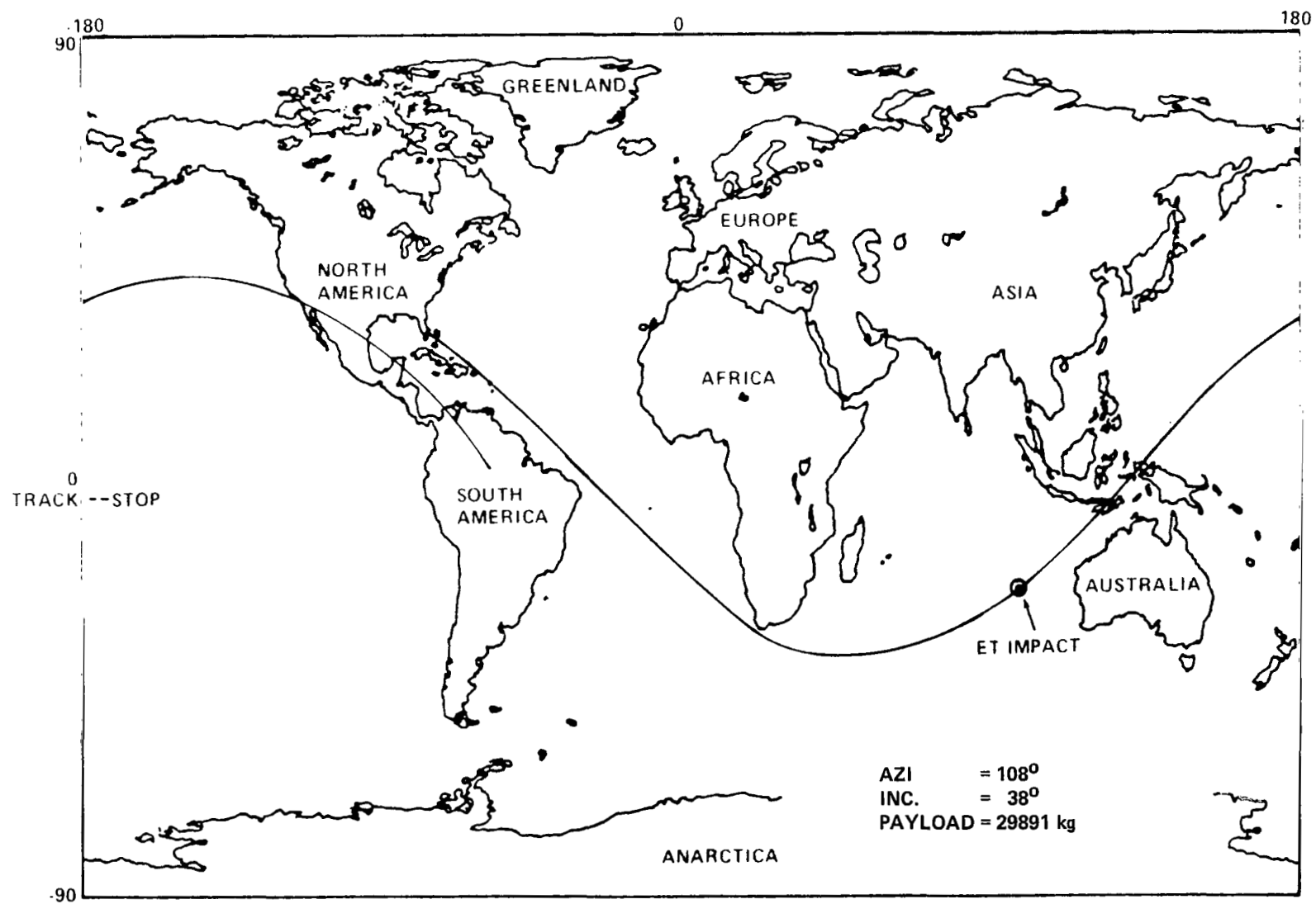
Figure 24. Orbiter/ET impact trace for ETR launch (yaw steering after SRB separation).
