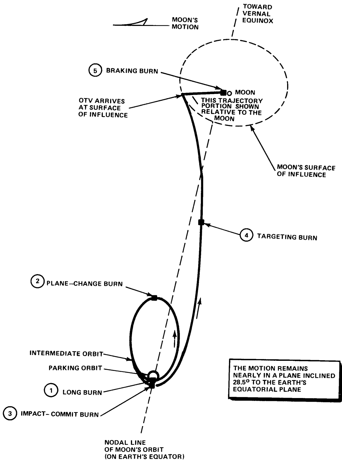
Figure 6. Flight profile for the lunar orbit mission.
