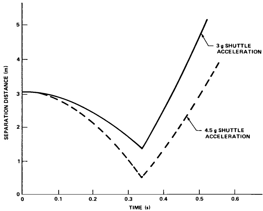
Figure 22. Orbiter/payload separation.
