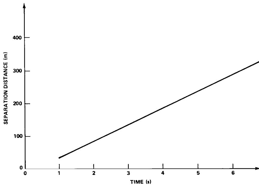
Figure 23. Orbiter/payload separation.
