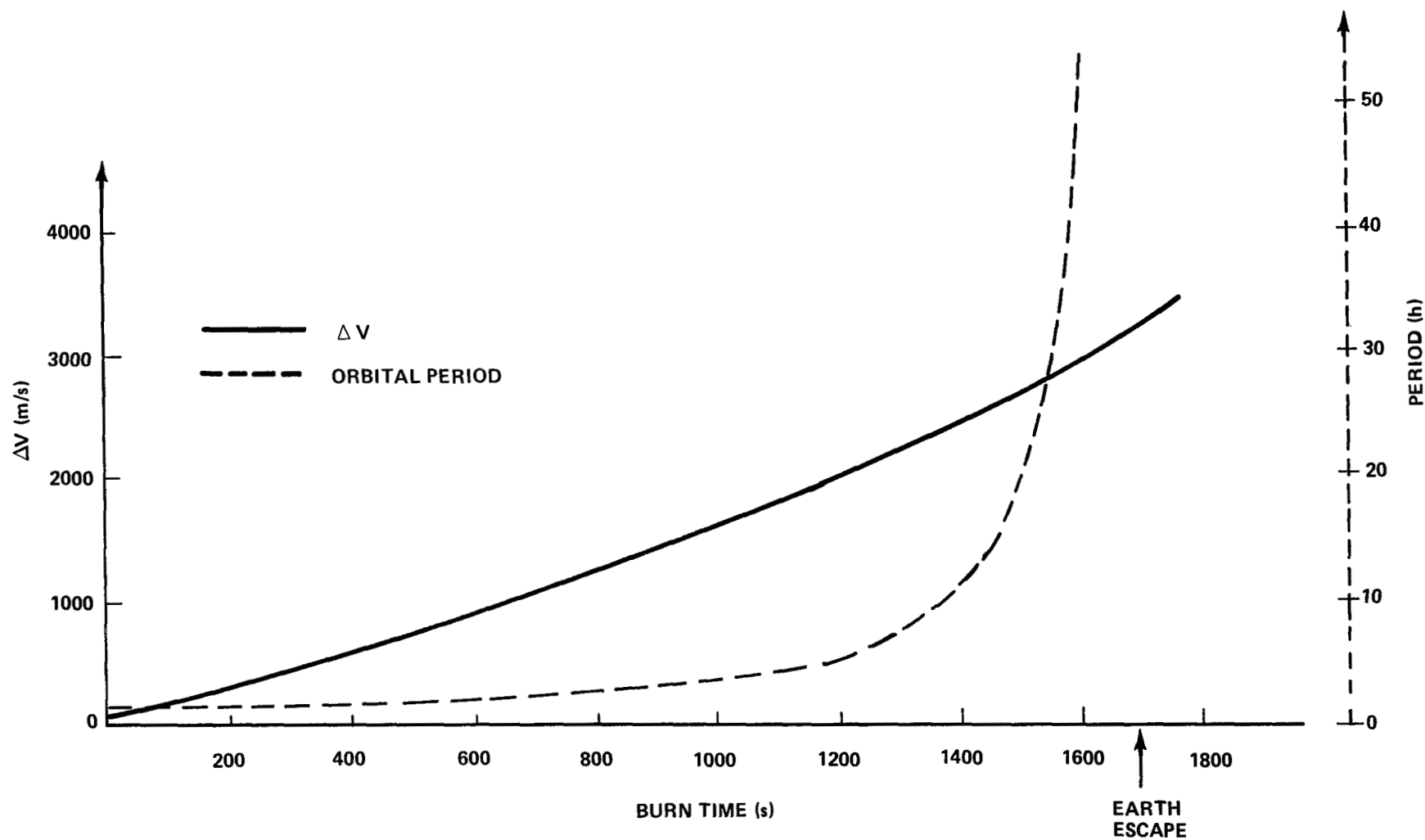
Figure 9. \Delta velocity and period versus OTV burntime for 0.86 AU mission.
