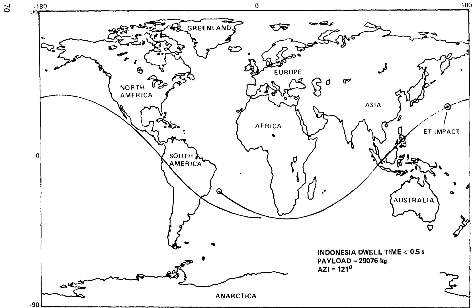
Figure 25. Orbiter/ET impact trace for Trindade launch.
