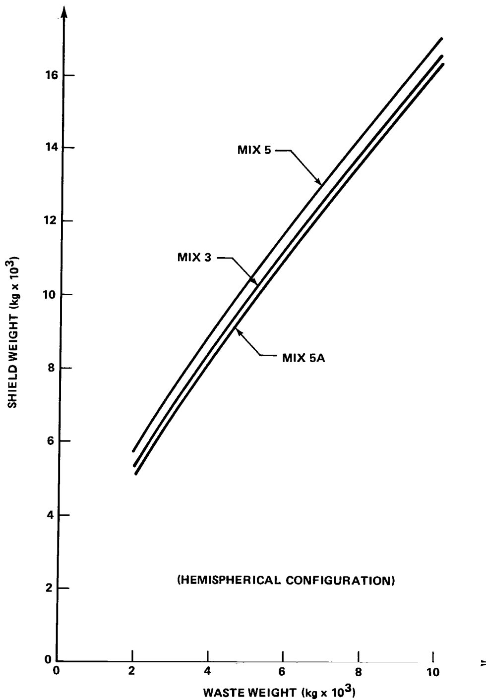
Figure 21. Shield weight for the different mixes (waste density = 4 \text{ gm/cm}^3 ).
