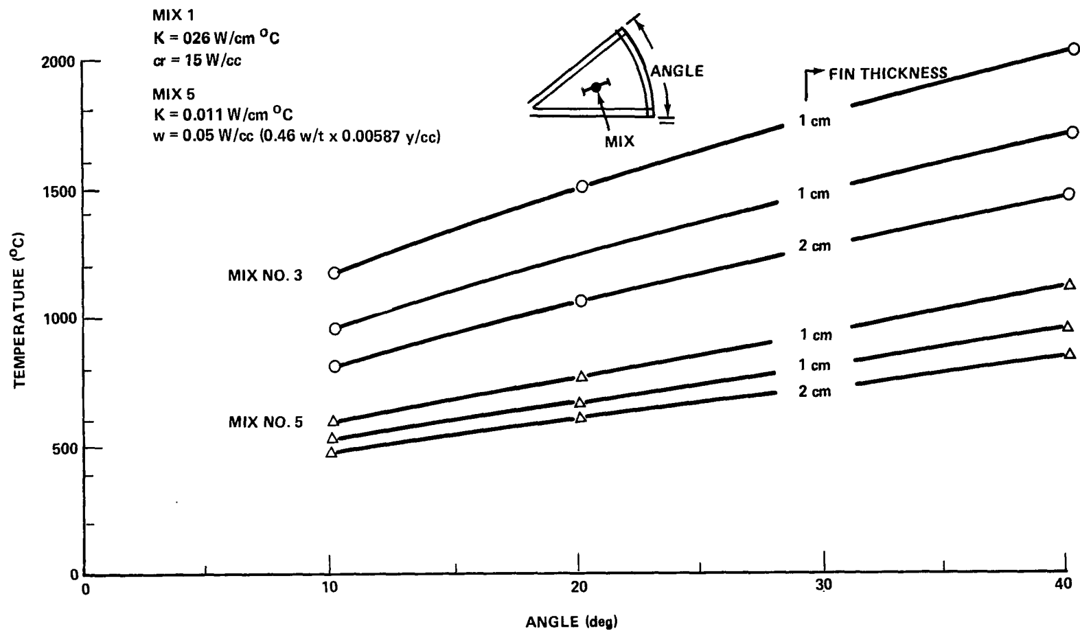
Figure 15. Nuclear waste maximum temperature versus angle between fins at various fin thicknesses.
