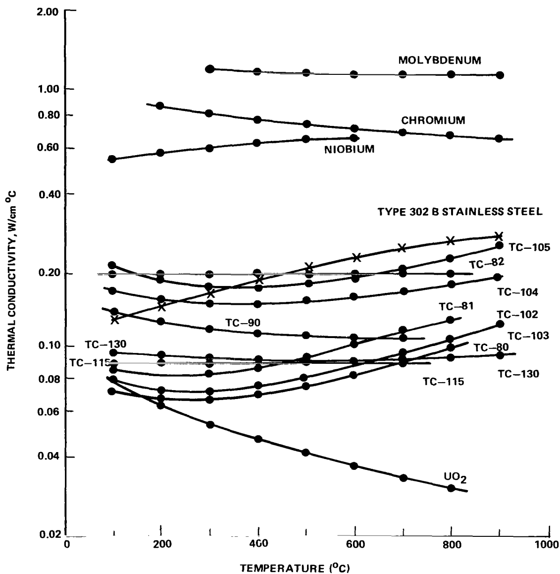
Figure 4. Thermal conductivity versus temperature for UO 2 cermet and their matrix metals.
