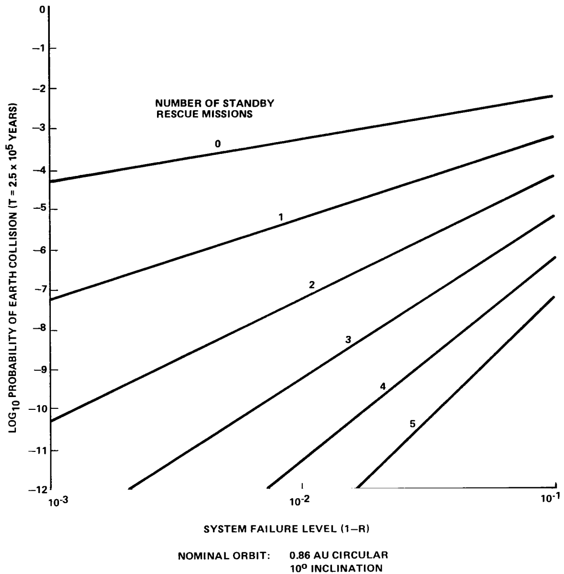
Figure 10. Risk profile for solar orbit disposal with retrieval.
