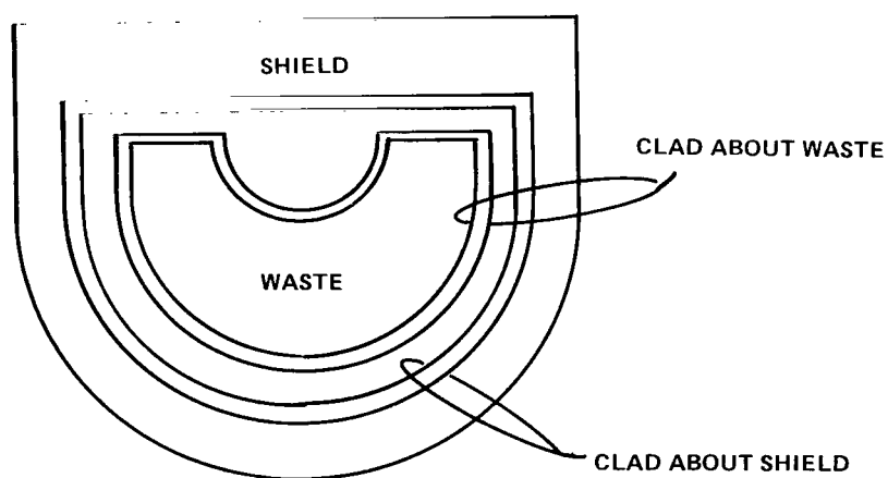
Figure 17. Typical shield for the hemispherical shield.
