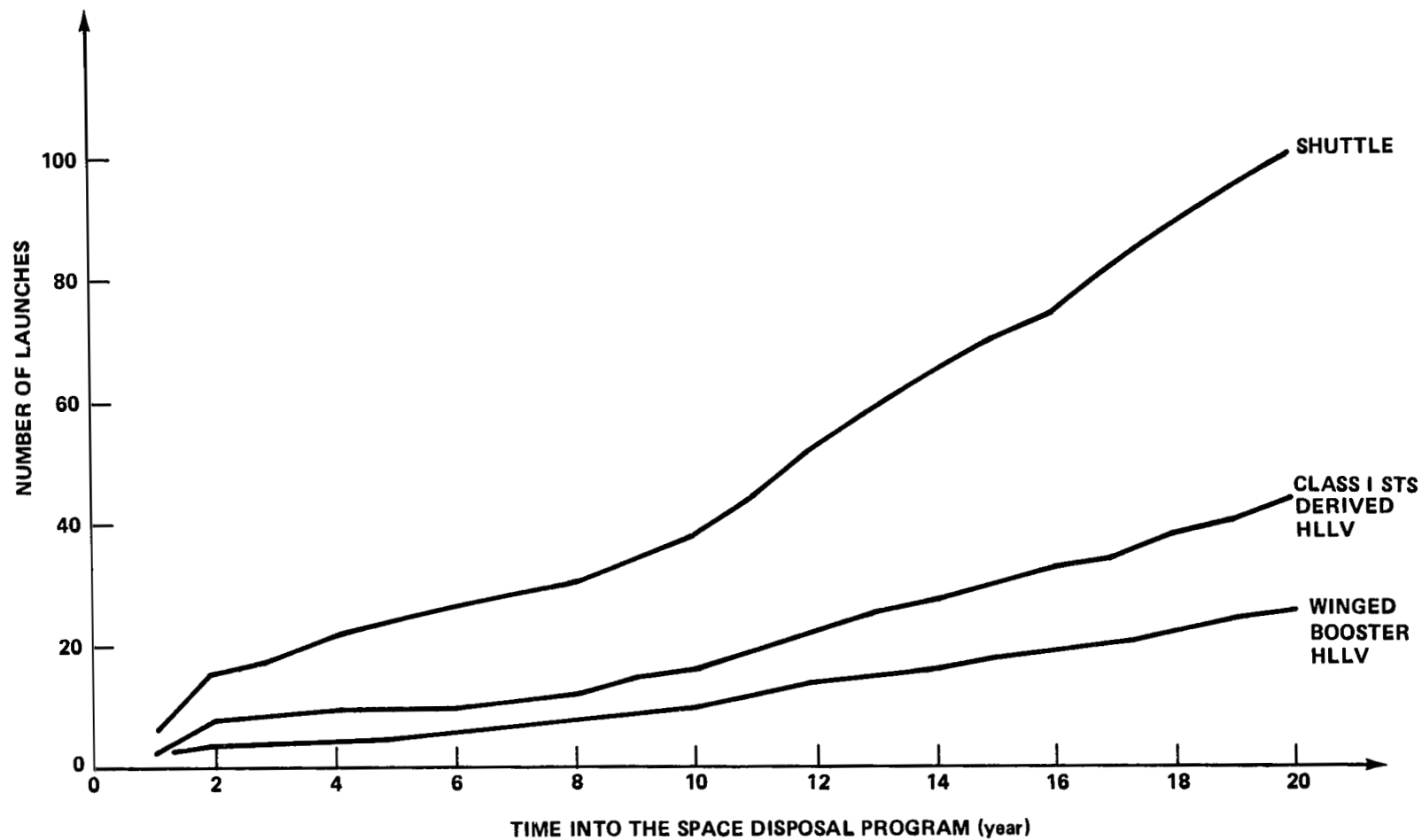
Figure 36. Launch rates for LSL mission (Mix 3).
