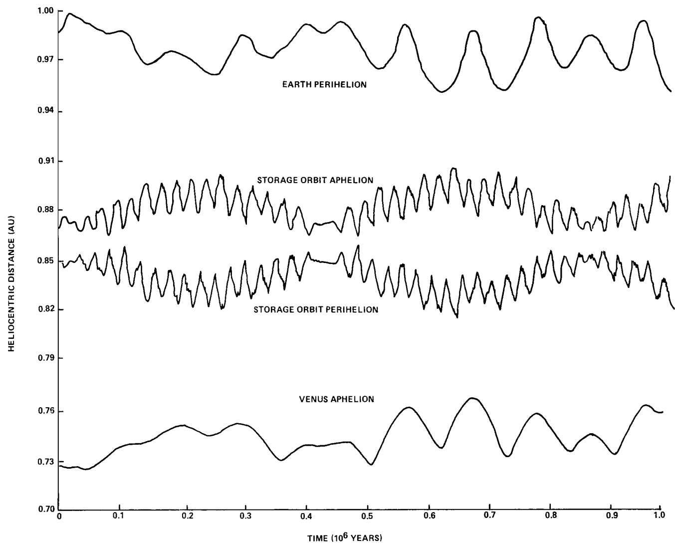
Figure 8. Long term variations in aphelion and perihelion.
