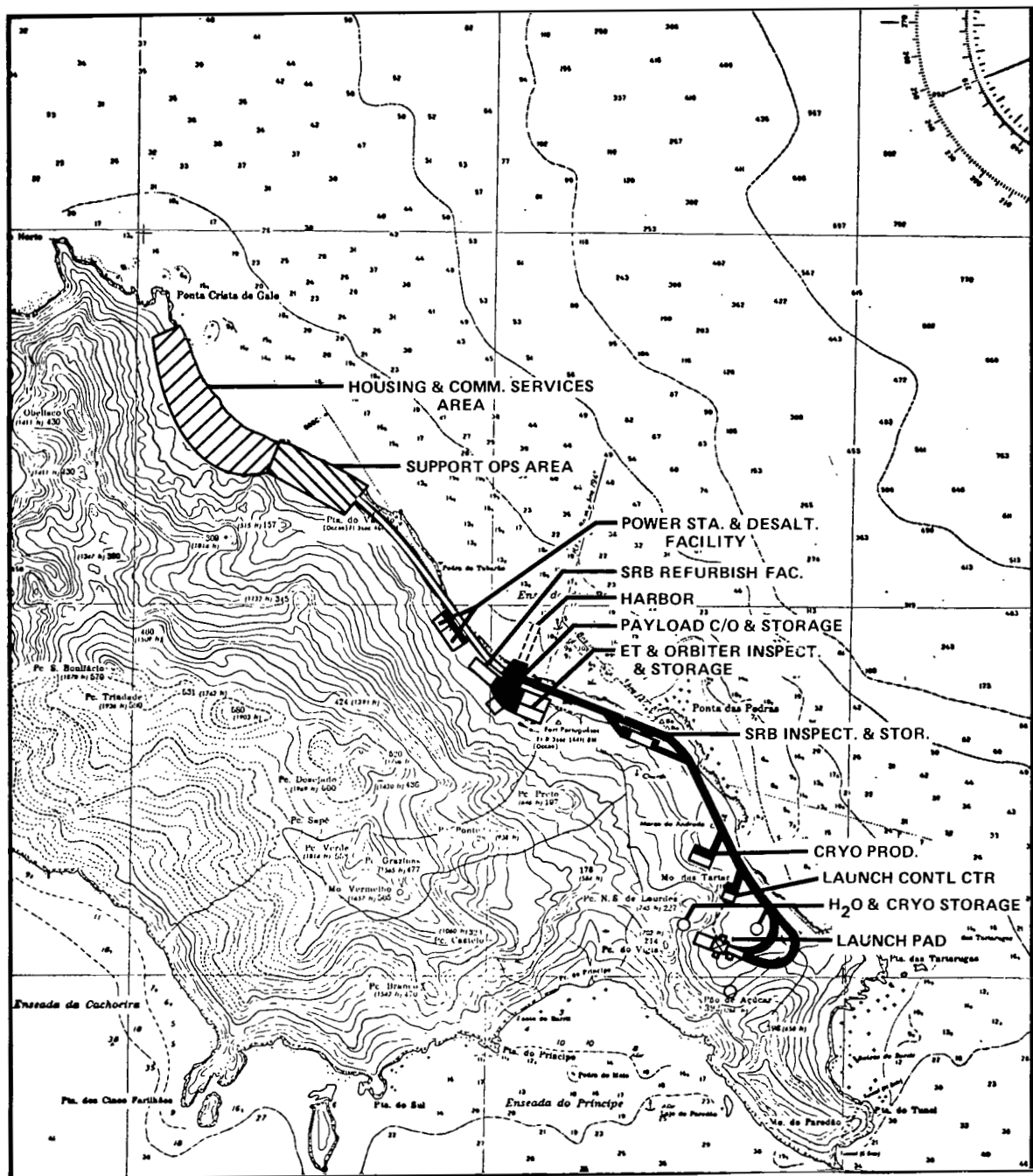
Figure 26. Remote operational base concept Trindade Island (Brazil).
