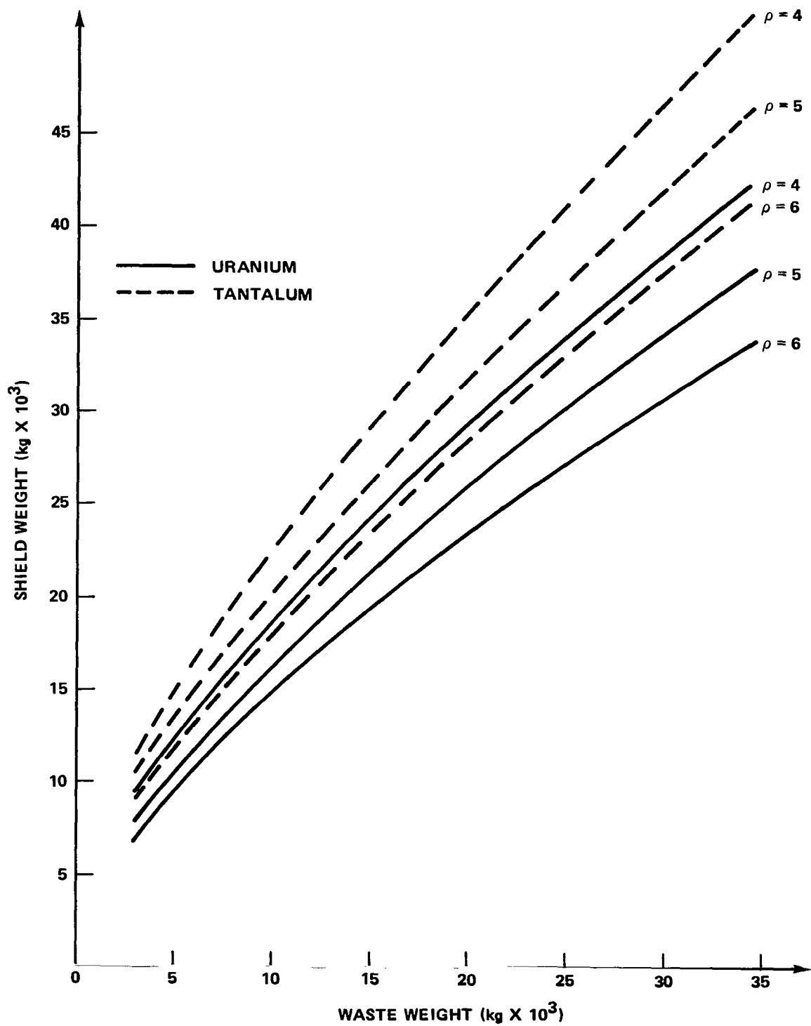
Figure 18. Shield weight for 19 cylinder configuration.
