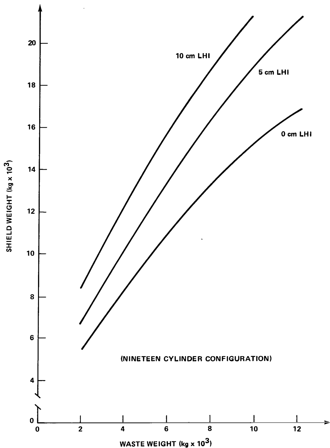
Figure 19. Neutron shielding effects.
