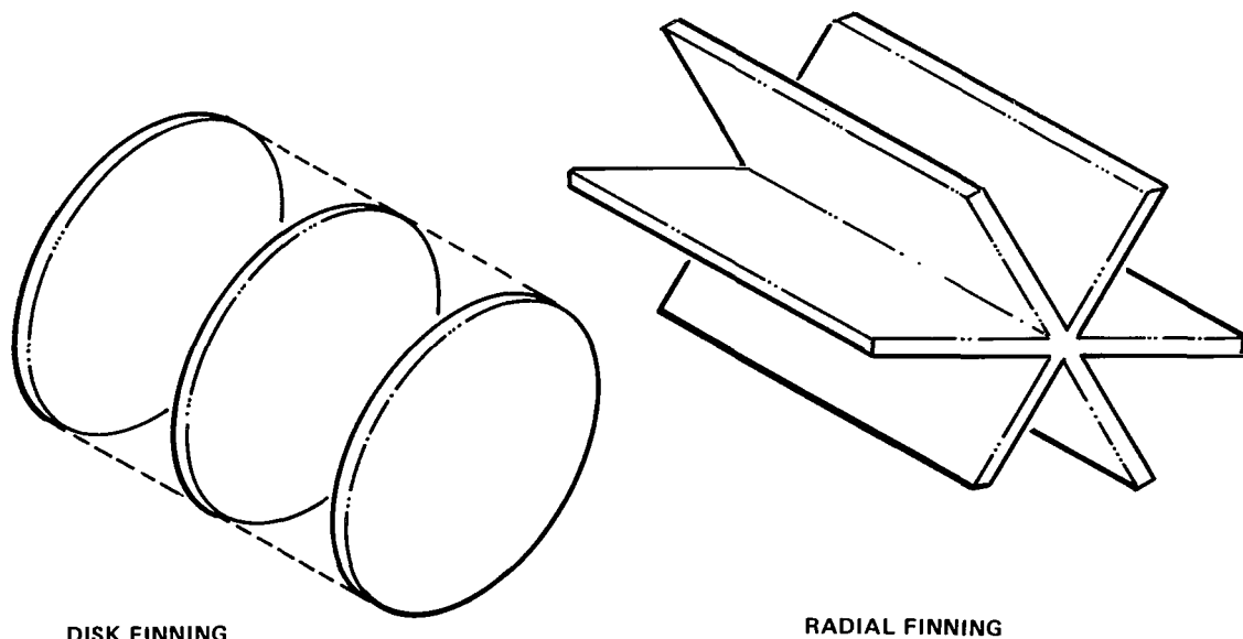
Figure 14. Radial and orthogonal finning concepts.
