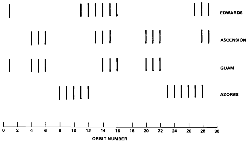
Figure 27. Deorbit opportunities for Trindade launch.
