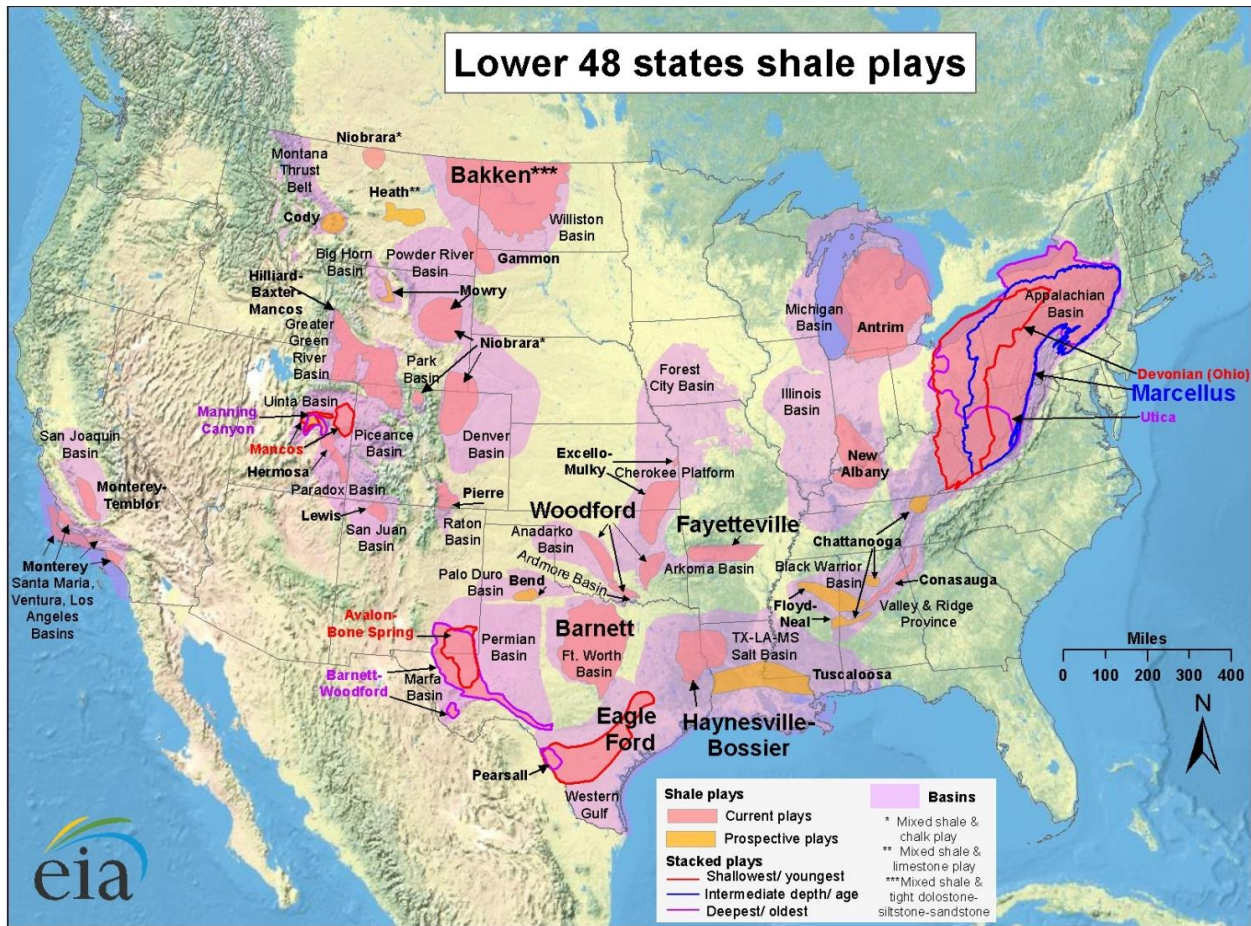
FIGURE 2 U.S. Shale Gas Plays (EIA, 2011)
