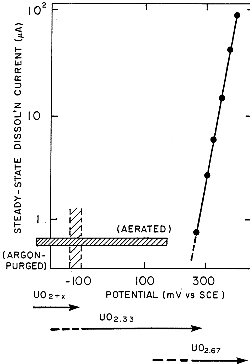
FIGURE D-1: Steady-State Currents as a Function of Applied Potential for the Anodic Dissolution of a UO_2 Electrode in 0.1 \text{ mol}\cdot\text{L}^{-1} NaClO_4 ( pH = 9.5 ) (from Shoosmith et al 1989). The horizontal bar shows the range of E_{CORR} values measured in the same solution in the presence of the various oxidants considered in this work. The horizontal arrows indicate the potential ranges for various surface compositions.
