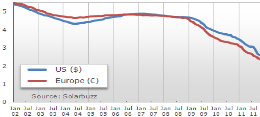
Figure 40. Solar Retail Module Price Index Solarbuzz Retail Module Price Index Dec 2001: $5.40 €5.47 — Nov 2011: $2.49 €2.33 Price per Watt Peak
