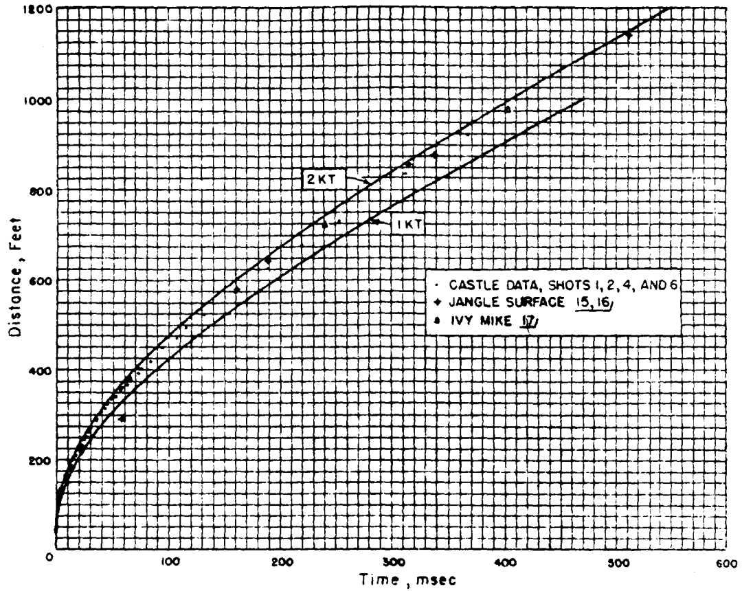
Figure 2.8 Surface arrival-time data scaled to 1 kt at sea level.
