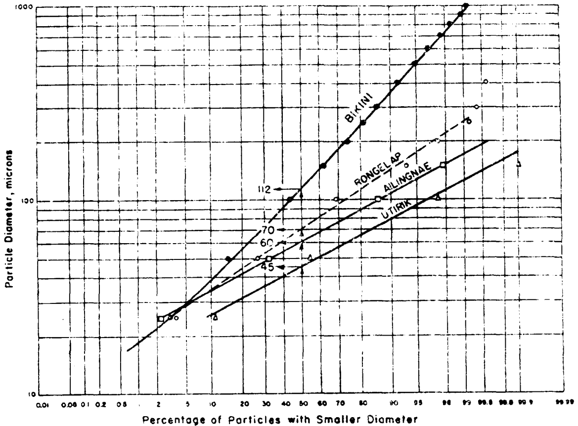
Figure 3.11 Cumulative particle-size distribution.
