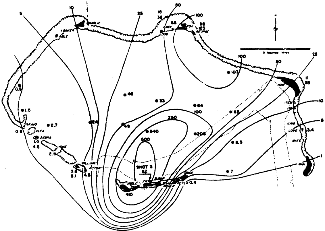
Figure 3.7 Close-in gamma fallout pattern, Shot 3, (r/hr at H + 1 hour).
