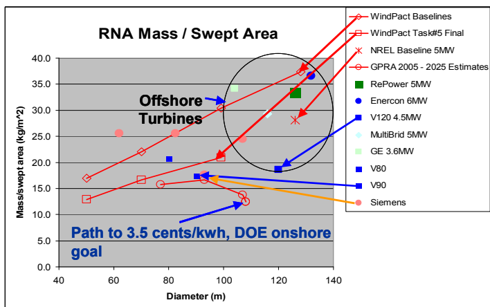
Figure 1: Impact of Maturing Technology and Innovation on Specific Rotor Nacelle Mass with Increasing Rotor Diameter
