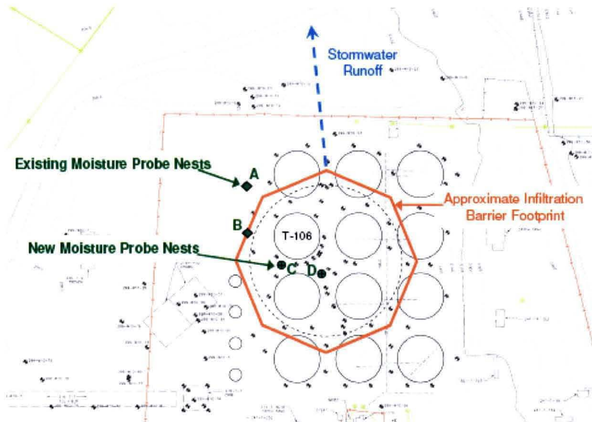
Fig. 4. Interim barrier being constructed in T Tank Farm
