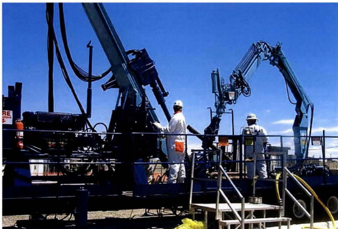
Fig. 1. Diesel hammer drill rig in SX Tank Farm
